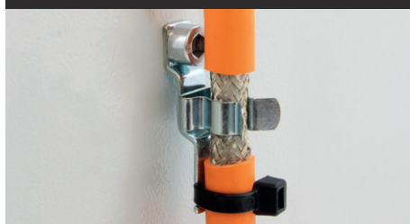
EMC shield clamp for screw assembly, with integrated strain relief function
